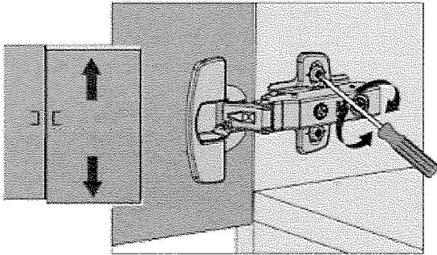
VERTICAL HINGE HEIGHT ADJUSTMENT
