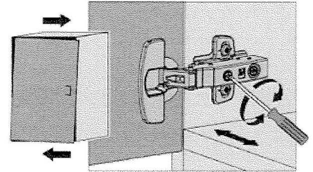
IN/OUT HINGE DEPTH ADJUSTMENT
